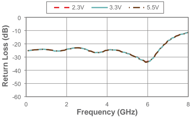
Figure 9 • Active Port Return Loss vs. Frequency
