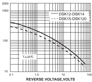
FIG. 5-TYPICAL JUNCTION CAPACITANCE
