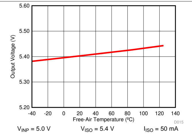
Figure 21. Isolated Supply Voltage ( V_{ISO} ) vs Free-Air Temperature
