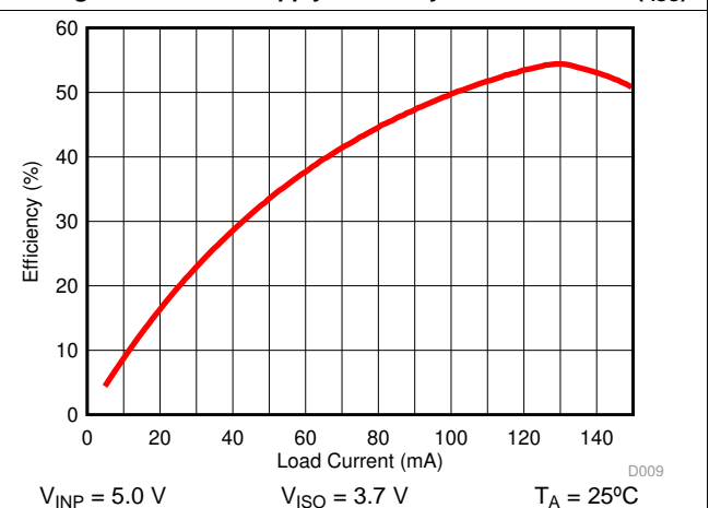
Figure 15. Power Supply Efficiency vs Load Current (I ISO )
