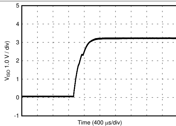
D056 Figure 52. V_{ISO} Soft Start at 90% Rated Load, 5.0-V Input, 3.3-V Output
