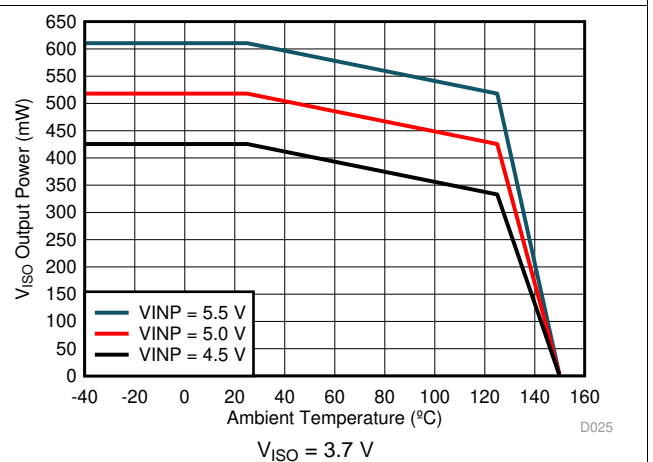
Figure 7. Maximum V ISO Output Power vs. Temperature
