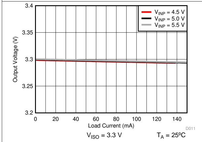
Figure 18. Isolated Supply Voltage ( V_{ISO} ) vs Load Current ( I_{iso} )
