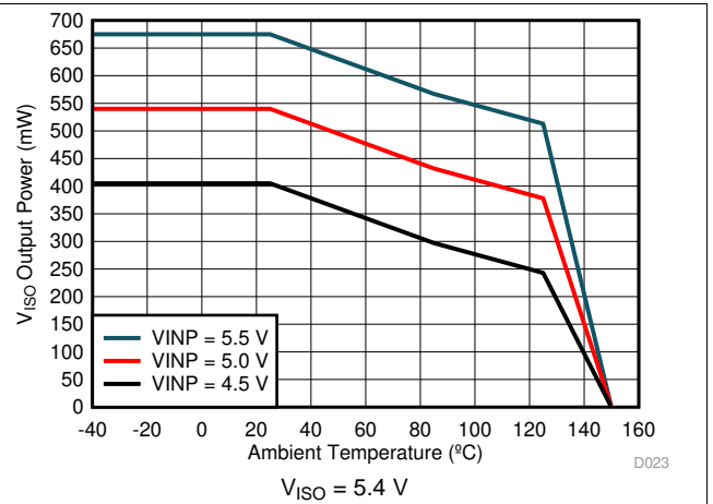
Figure 5. Maximum V ISO Output Power vs. Temperature
