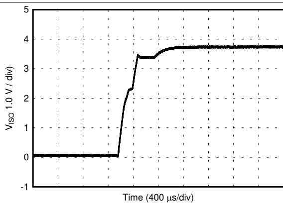
D053 Figure 49. V_{ISO} Soft Start at 10% Rated Load, 5.0-V Input, 3.7-V Output
