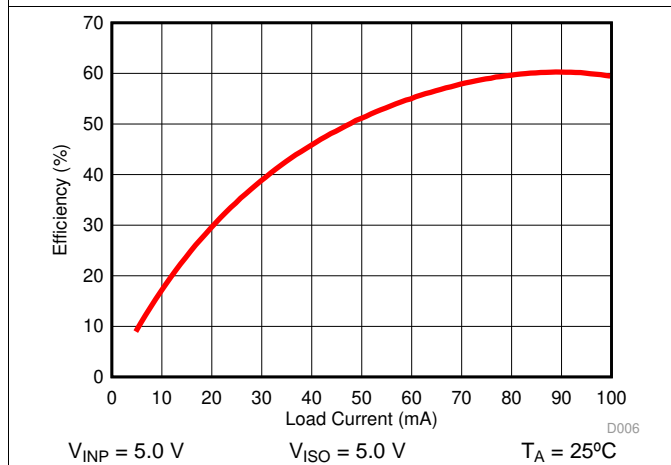
Figure 12. Power Supply Efficiency vs Load Current (I ISO )
