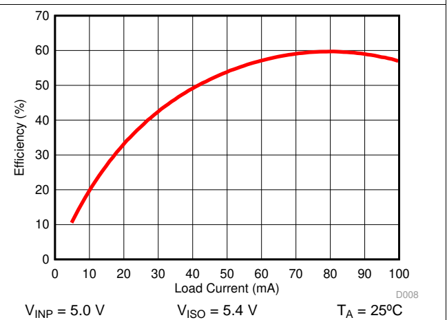
Figure 13. Power Supply Efficiency vs Load Current (I ISO )
