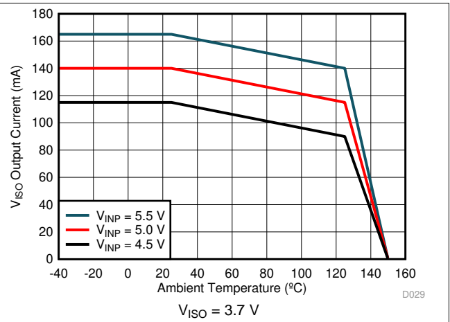
Figure 11. Maximum V ISO Output Current vs. Temperature
