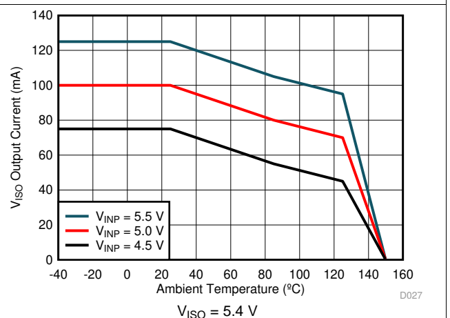
Figure 9. Maximum V ISO Output Current vs. Temperature
