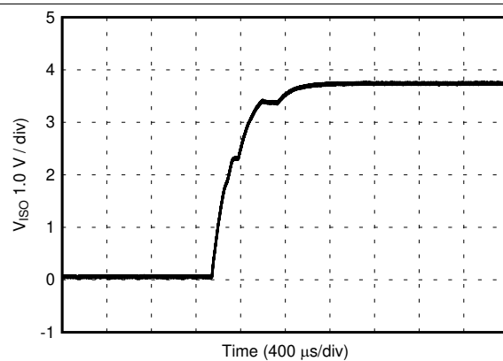
D054 Figure 50. V_{ISO} Soft Start at 90% Rated Load, 5.0-V Input, 3.7-V Output
