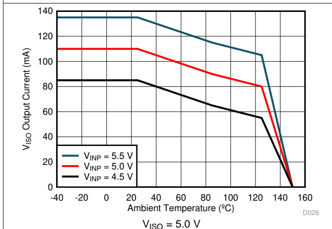
Figure 8. Maximum V ISO Output Current vs. Temperature
