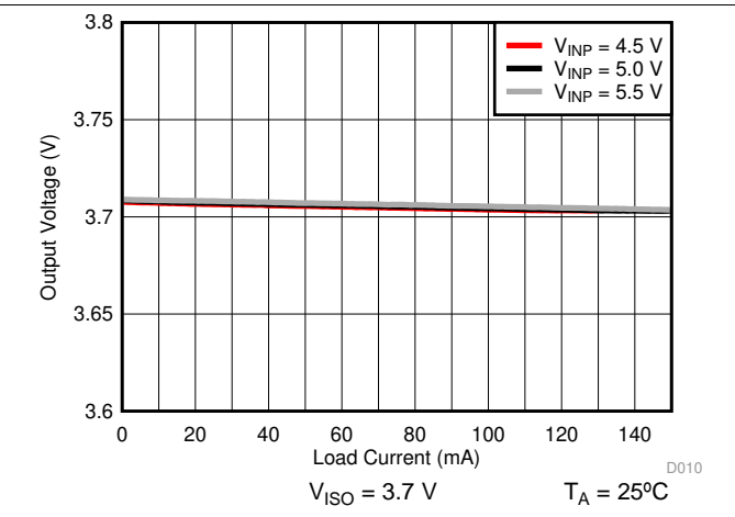
Figure 19. Isolated Supply Voltage ( V_{ISO} ) vs Load Current ( I_{iso} )
