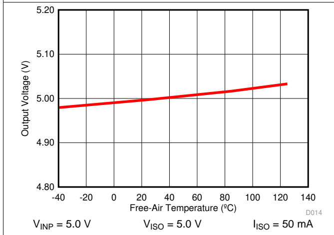
Figure 20. Isolated Supply Voltage ( V_{ISO} ) vs Free-Air Temperature
