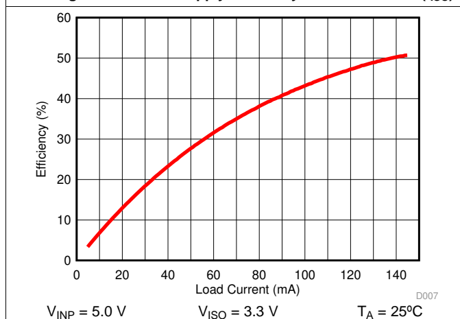
Figure 14. Power Supply Efficiency vs Load Current (I ISO )
