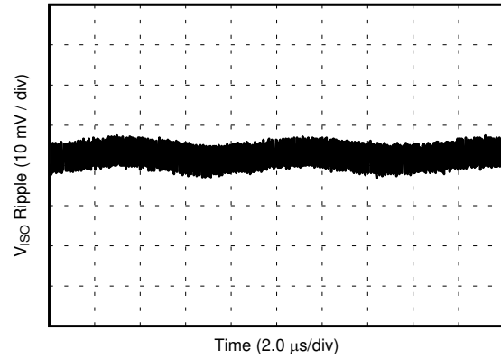
Figure 36. V_{ISO} Ripple, 3.3-V Output, 90% Load
