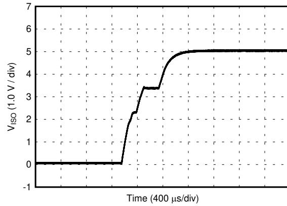
D052 Figure 48. V_{ISO} Soft Start at 90% Rated Load, 5.0-V Input, 5.0-V Output
