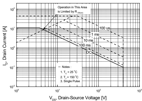
Figure 9-2. Maximum Safe Operating Area for TSF740MR
