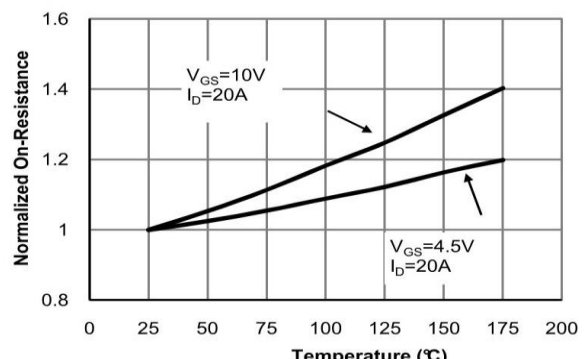
Figure 4: On-Resistance vs. Junction Temperature (Note E)
