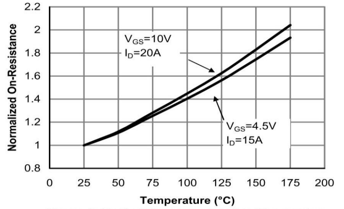
Figure 4: On-Resistance vs. Junction Temperature (Note E)
