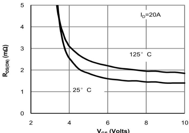
Figure 5: On-Resistance vs. Gate-Source Voltage (Note E)
