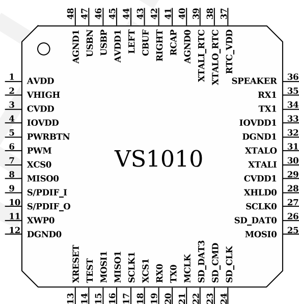
Figure 2: VS1010d pins, LQFP-48
