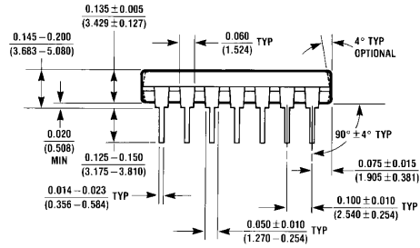
14-Lead Molded Dual-In-Line Package (N) Order Number DM74LS02N NS Package Number N14A
