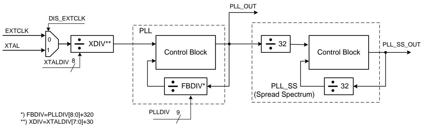
Figure 5. PLL Block Diagram
