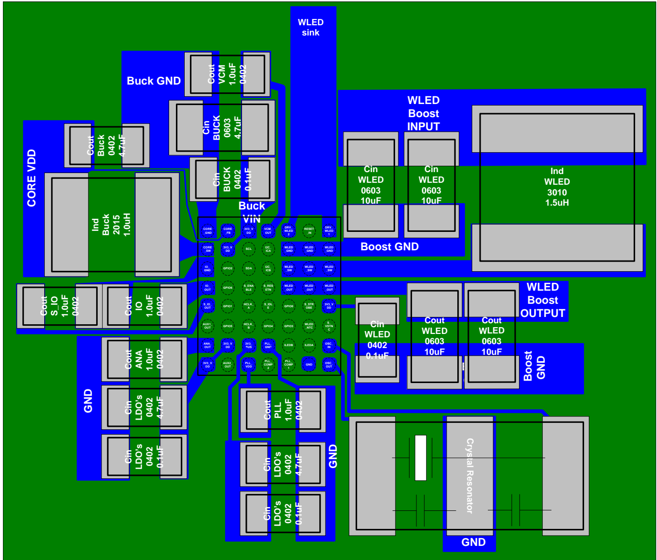
Figure 92. Layout
