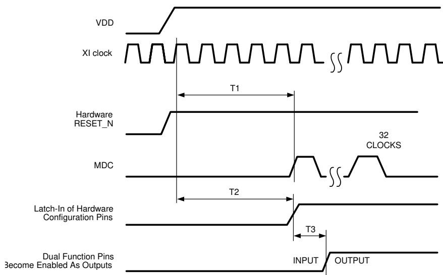
Figure 1. Power-Up Timing
