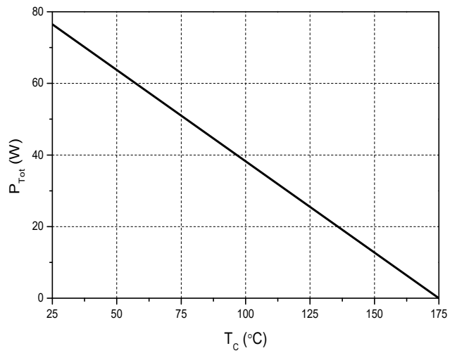
Figure 6. Power Derating
