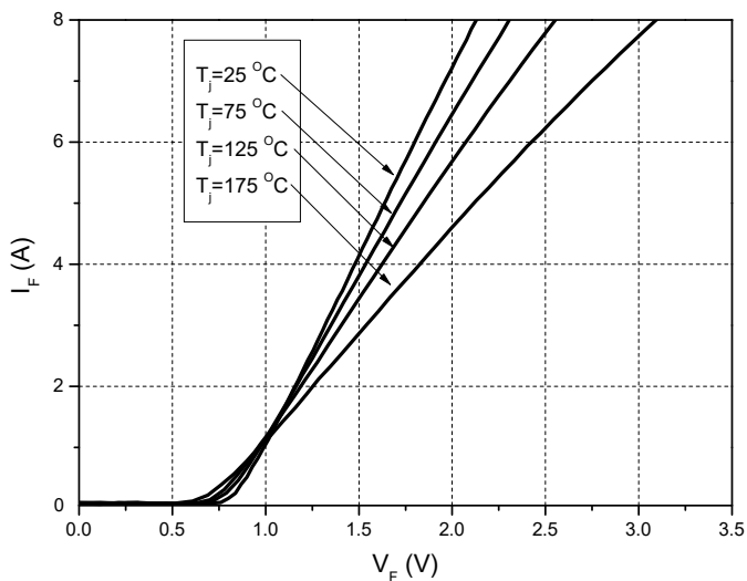
Figure 1. Forward Characteristics
