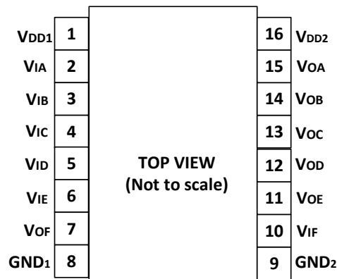
Figure4. \pi 161Mxx Pin Configuration
