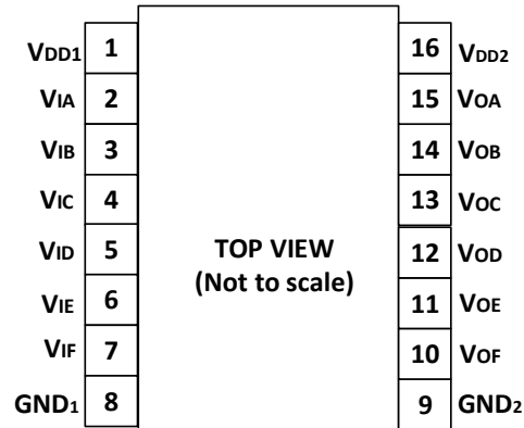
Figure3. \pi 160Mxx Pin Configuration
