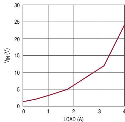
最小 V IN 与负载的关系曲线， V OUT = -8V
