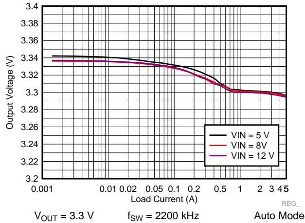
Figure 45. LM73605 Load and Line Regulation
