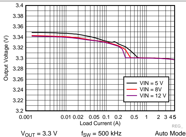
Figure 47. LM73605 Load and Line Regulation
