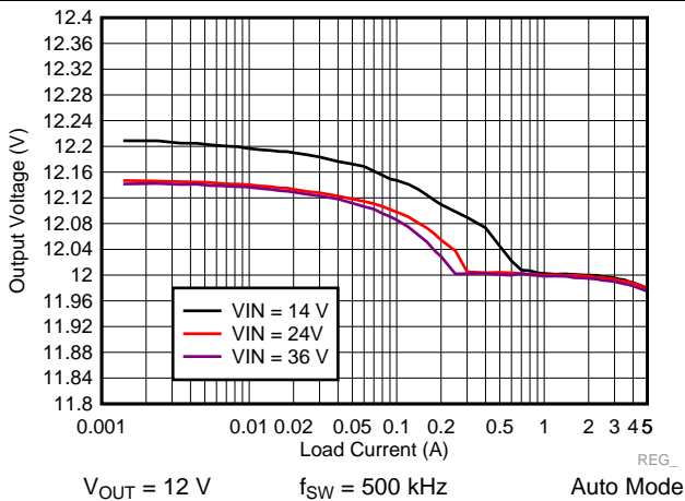
Figure 49. LM73605 Load and Line Regulation
