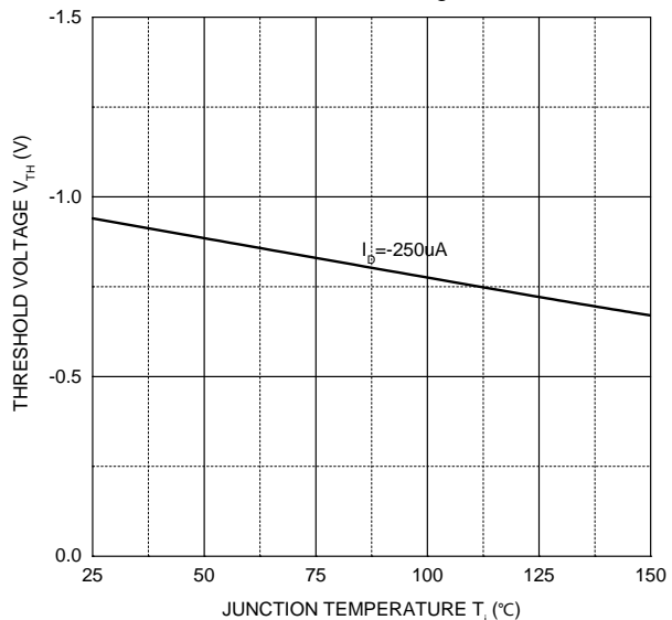
Threshold Voltage
