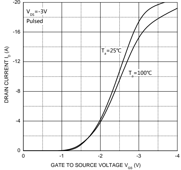
Transfer Characteristics
