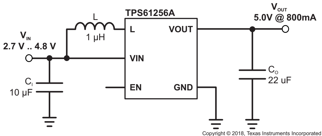
Figure 14. Typical Application
