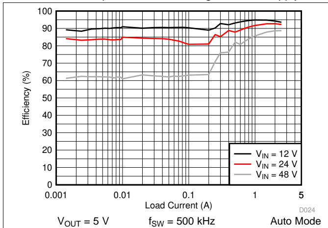
Figure 35. LM76002 Efficiency
