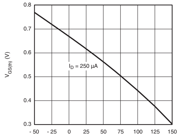
Threshold Voltage
