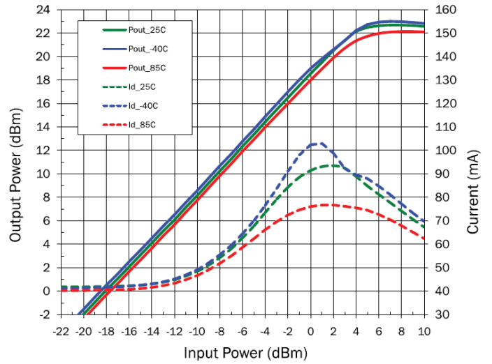
Output Power versus Input Power ( V_D = 5 V)
