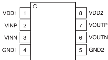
Pin Functions
