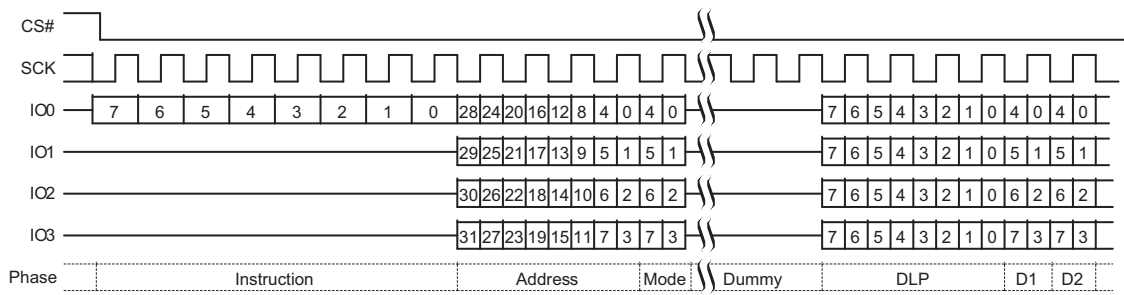
Figure 14. DDR Quad I/O Read
