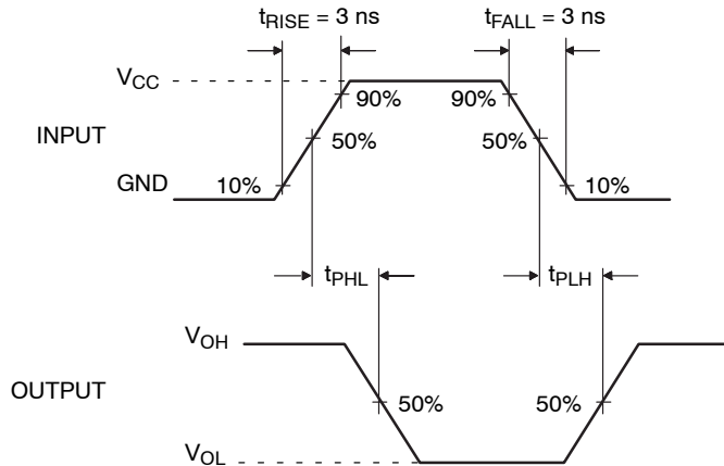
Figure 7. AC Waveforms
