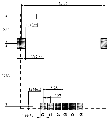
PCB LAYOUT
