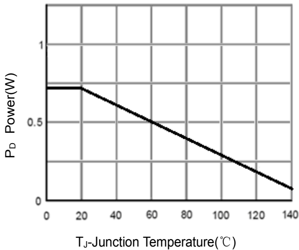
Figure 3 Power Dissipation
