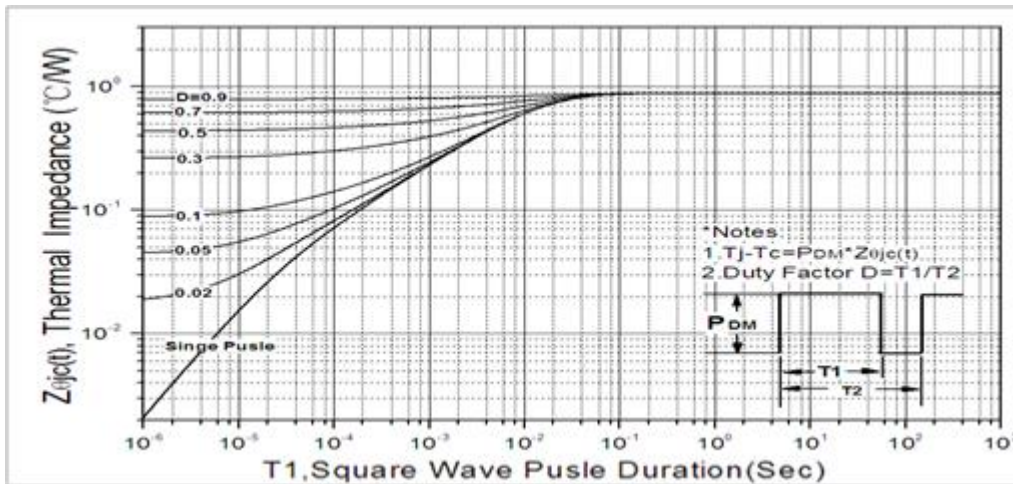
Fig. 19. Transient thermal response curve(TO-251&TO-251N)
