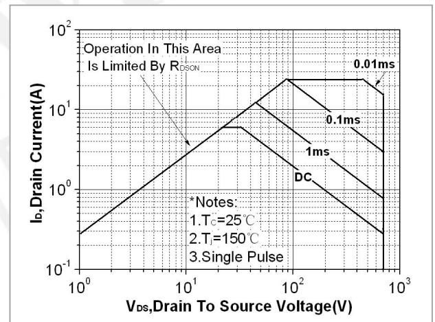
Fig. 12. Maximum safe operating area(TO-251&TO-251N)
