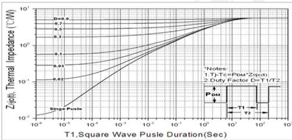
Fig. 18. Transient thermal response curve(TO-220F)
