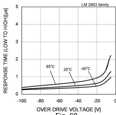
Fig. 60 Response Time (Low to High) – Over Drive Voltage (VCC=5[V],VRL=5[V],RL=5.1[kΩ])
