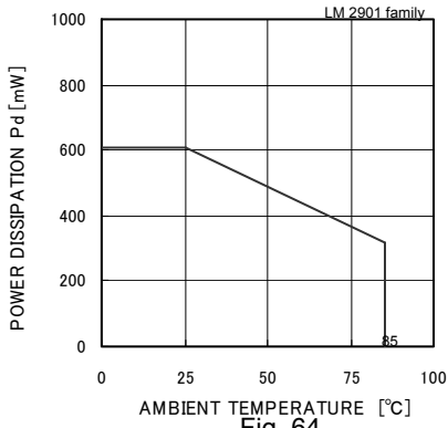
Fig. 64 Derating Curve
