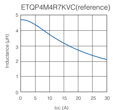
● Fig.1 Inductance v.s. DC current
