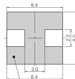
Series PCC-M0748M-LE (ETQP4M□□□KFM)
