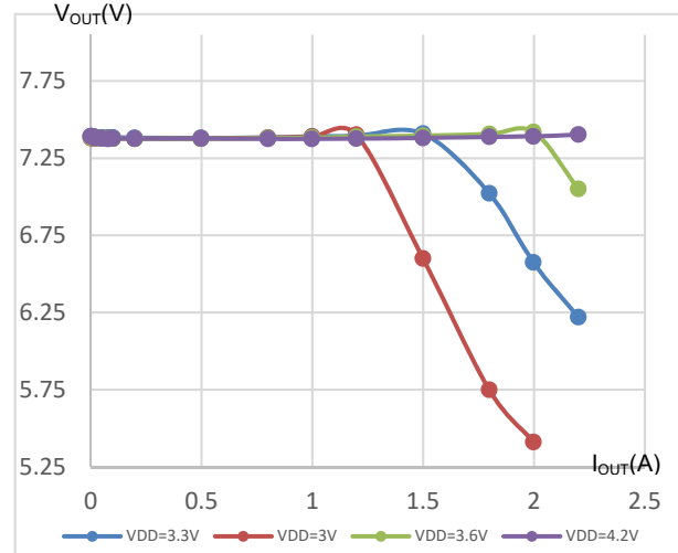
Load Regulation
