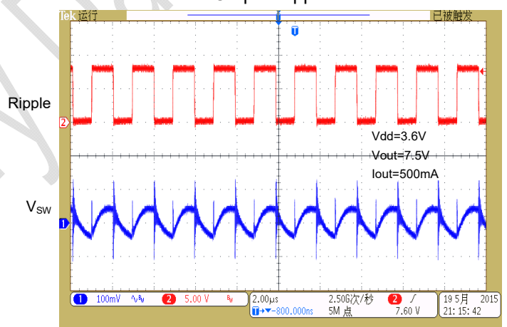
Output Ripple
