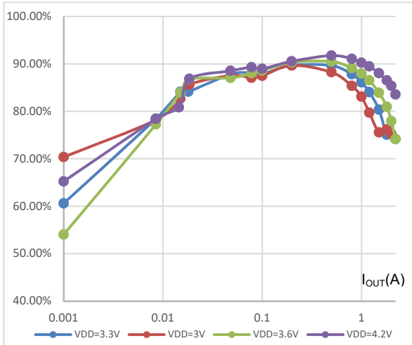
Efficiency
