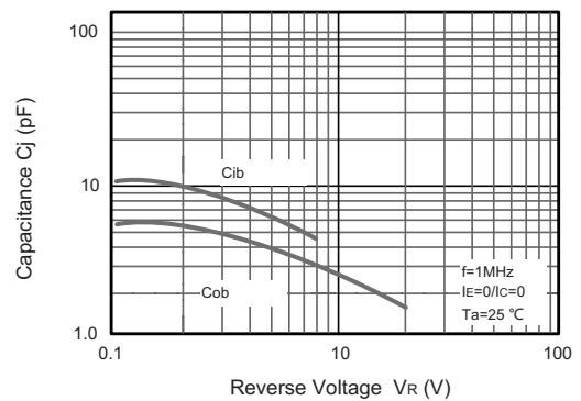
Fig.8 C_{ob}/C_{ib}-V_{CB}/V_{EB}
