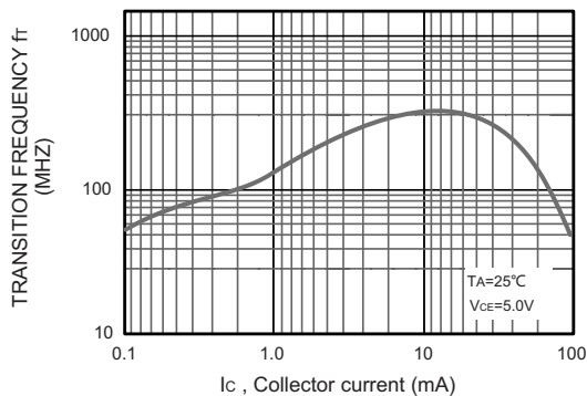
Fig.7 f_T-I_C
