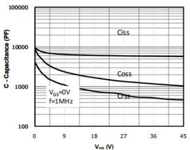
Fig 6: Capacitance Characteristics
