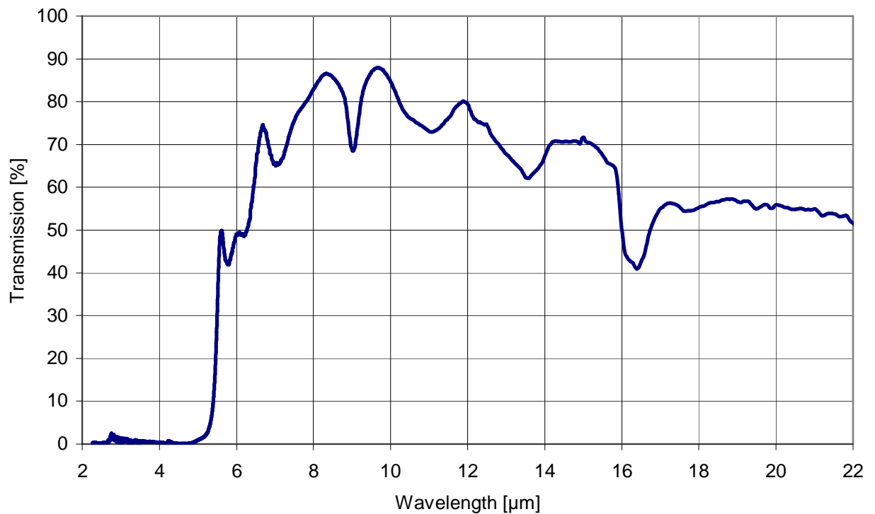
Typical Transmission 5.5µm Filter
