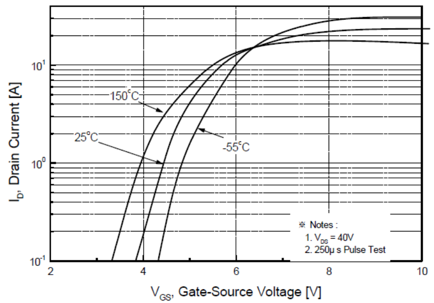
Figure 2. Transfer Characteristics
