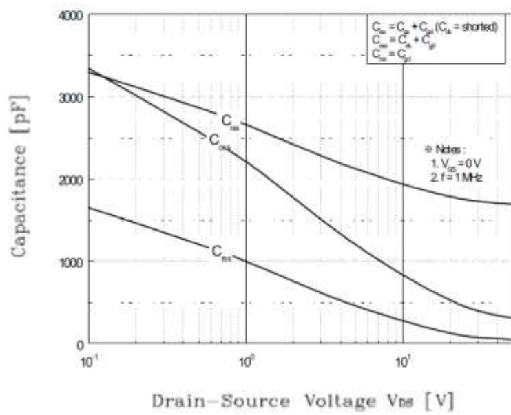
Figure 5. Capacitance Characteristics
