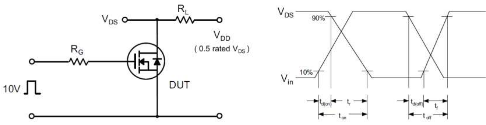
Fig 13. Resistive Switching Test Circuit & Waveforms
