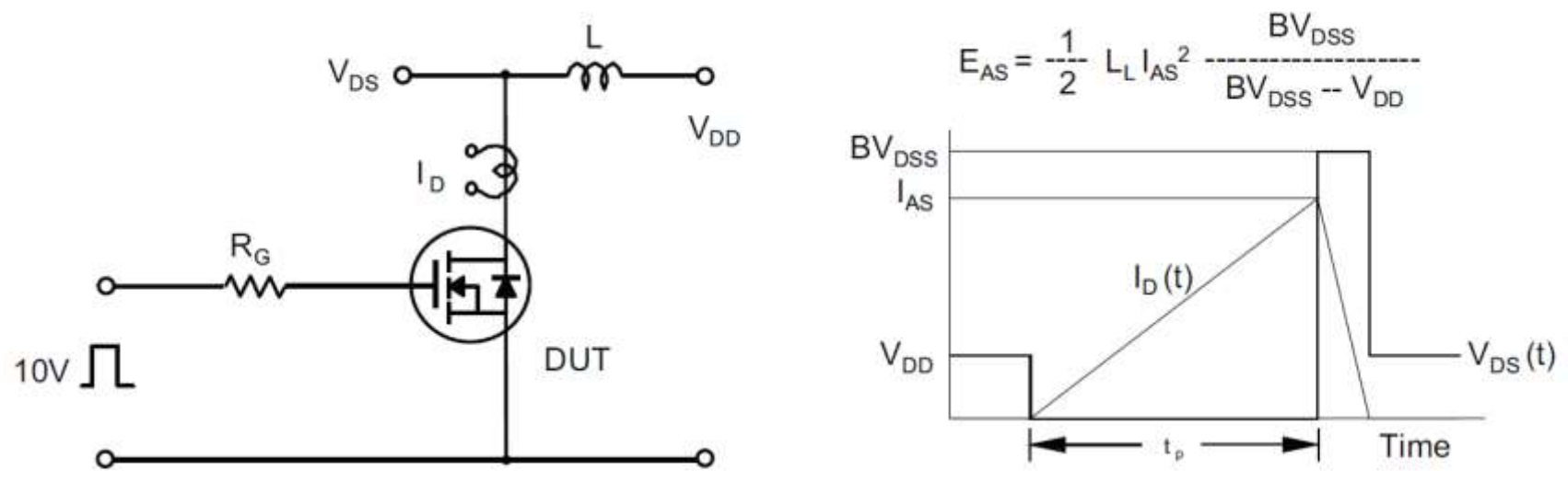
Fig 14. Unclamped Inductive Switching Test Circuit & Waveforms
