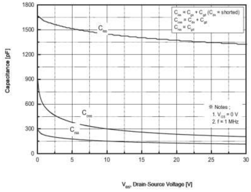
Fig.8 Capacitance Characteristics
