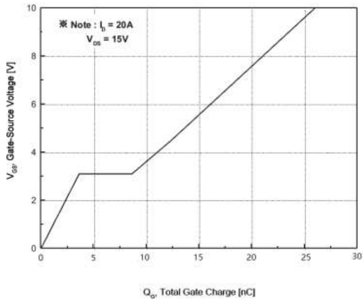
Fig.7 Gate Charge Characteristics
