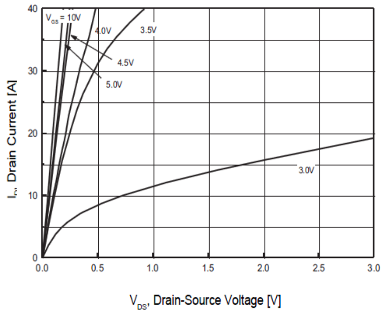
Fig.1 On-Region Characteristics
