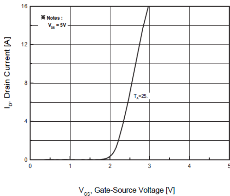
Fig.5 Transfer Characteristics
