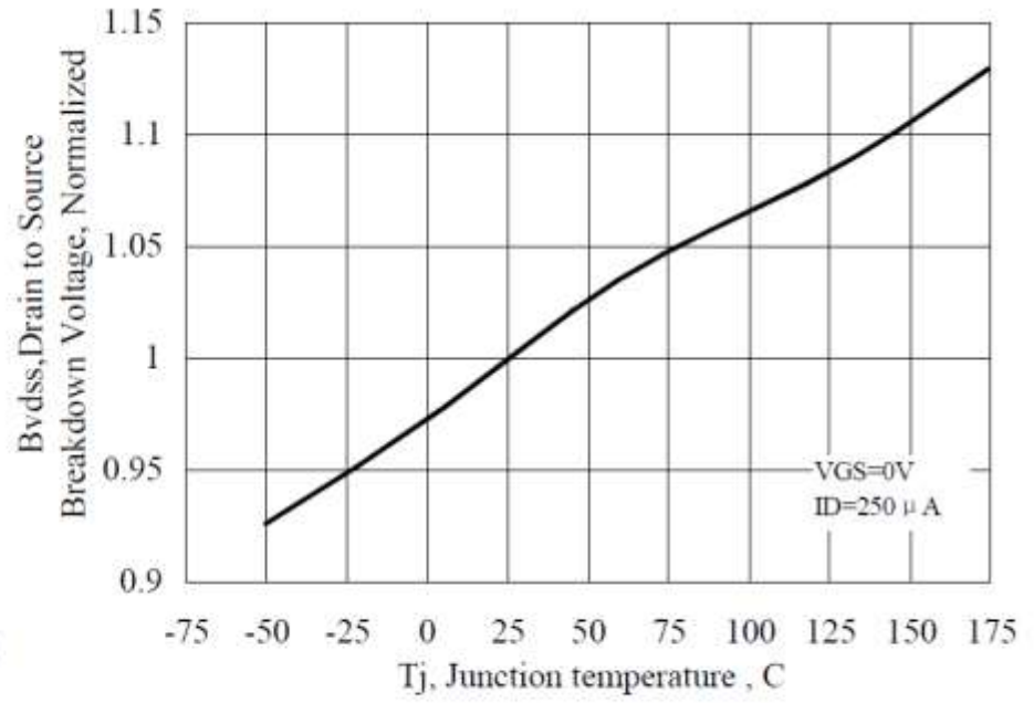
Figure 12 Typical Breakdown Voltage vs Junction Temperature
