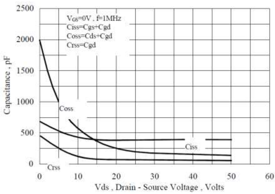
Figure 13 Typical Capacitance vs Drain to Source Voltage
