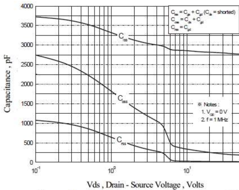
Figure 13 Typical Capacitance vs Drain to Source Voltage
