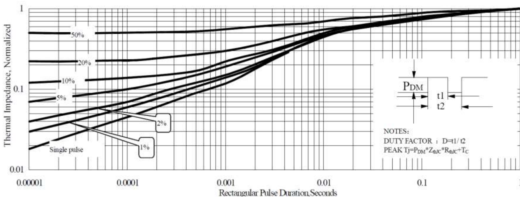
Figure 5 Maximum Effective Thermal Impedance, Junction to Case
