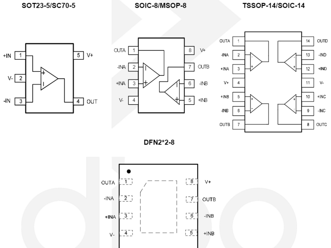
Figure 1 Pin Assignment
