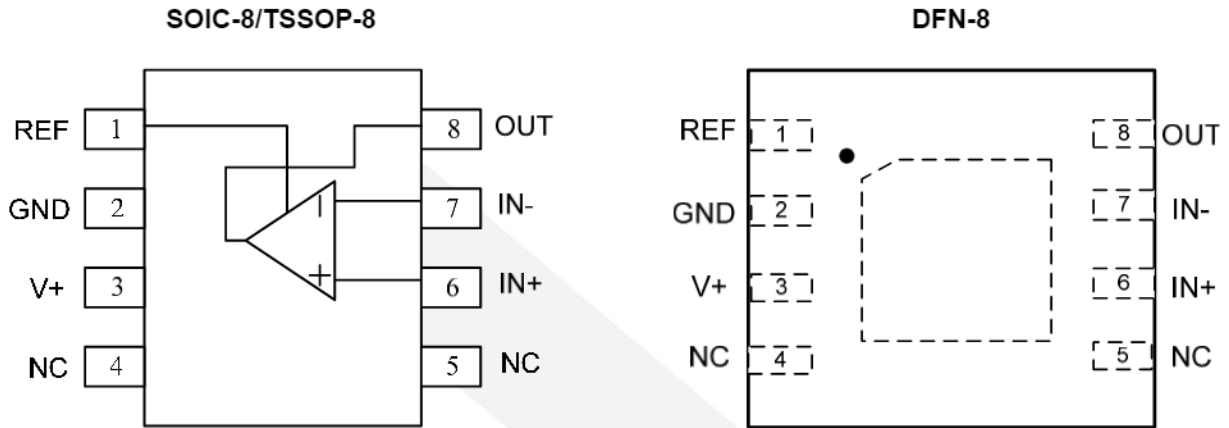
Figure 1 Pin Assignment
