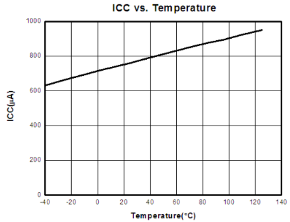
ICC & Temperature
