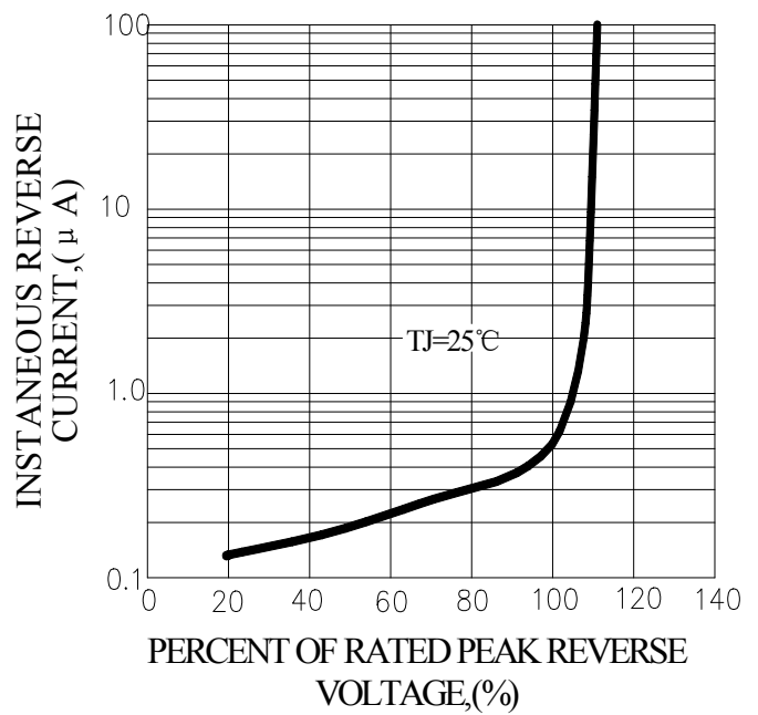
FIG.4-TYPICAL REVERSE CHARACTERISTICS
