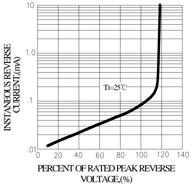
FIG.4-TYPICAL REVERSE CHARACTERISTICS
