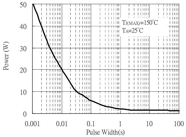
Single Pulse Power Rating, Junction to Ambient (Note 1 on page 1)
