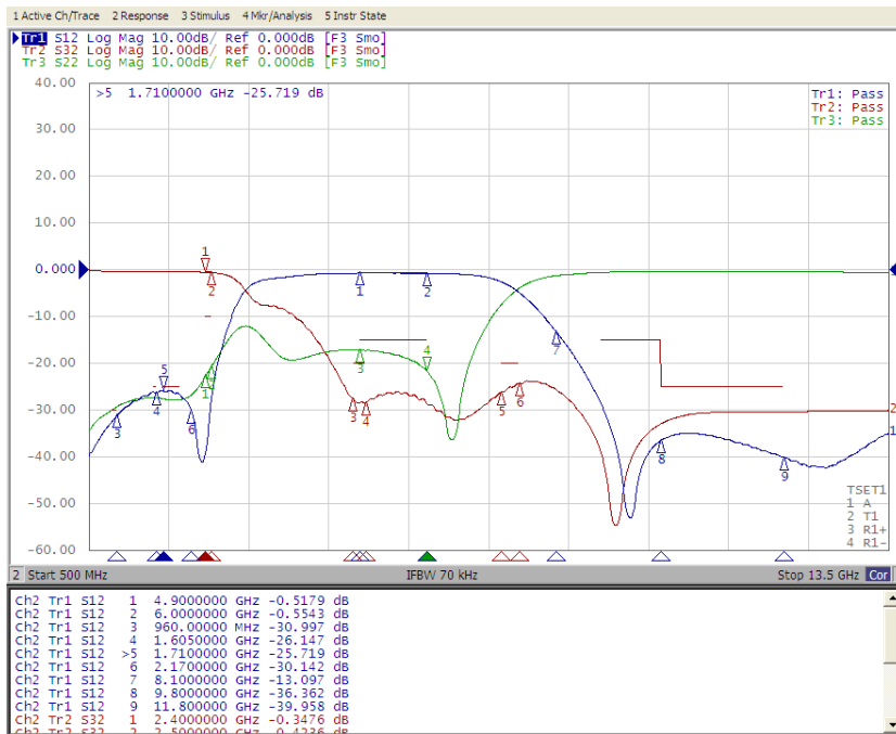
Fig.3 Frequency Characteristics
