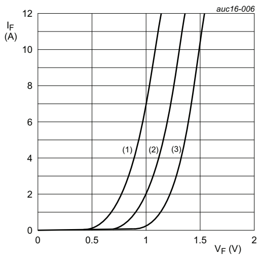
V 0 = 0.992 V; R s = 0.0327 Ω (1) T j = 150 °C; typical values (2) T j = 150 °C; maximum values (3) T j = 25 °C; maximum values
