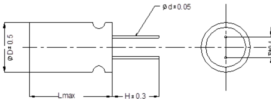
Figure 2 Dimension
