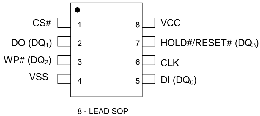
Figure.1 CONNECTION DIAGRAMS
