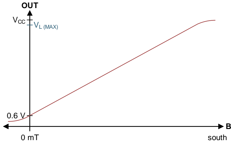
Figure 16. Magnetic Response
