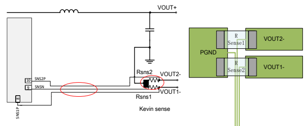
Figure.9 Current sense
